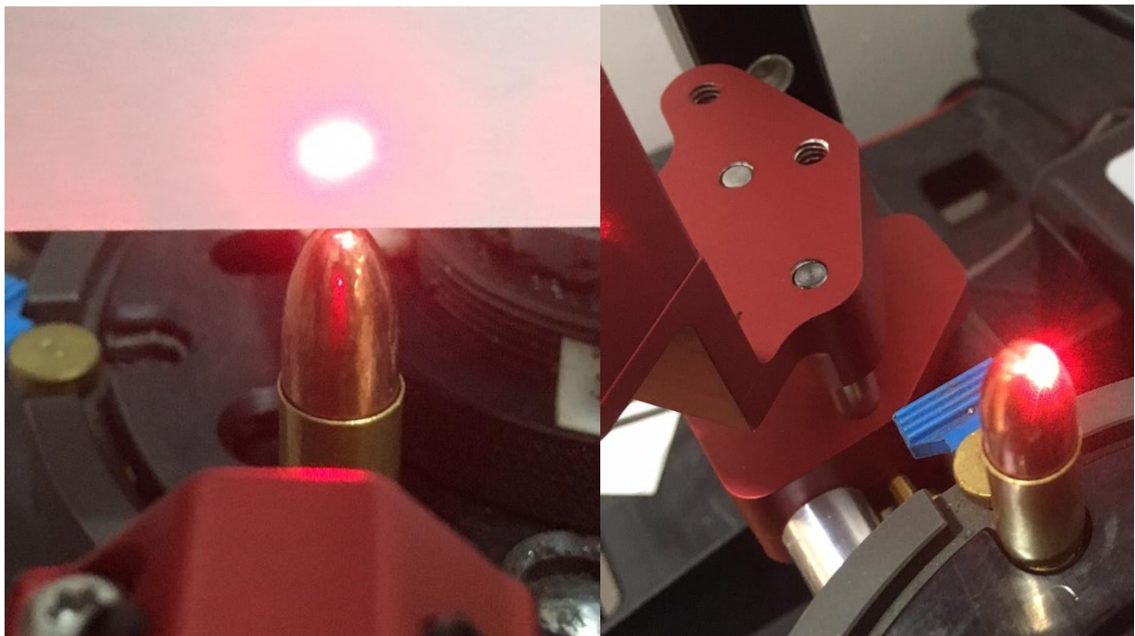
Figure 48: Direct beam over the tip of the bullet (left) the reflected beam will hit the back side of the bullet (Right)
