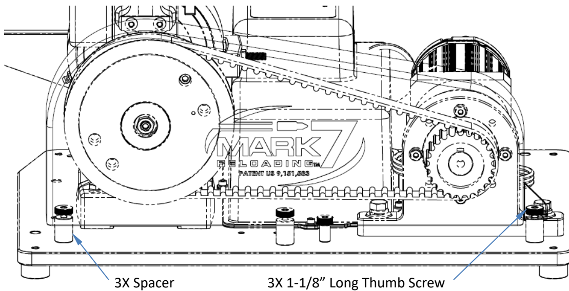
Figure 7: Belt Guard Installed (RL 1100/CP2000)
