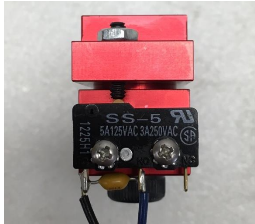
Figure 34: Micro switch Adjustment
