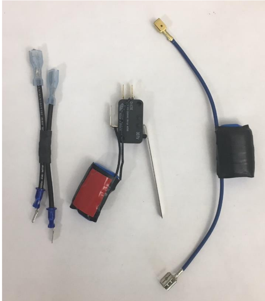
Figure 17: Case Feeder RC Filter
