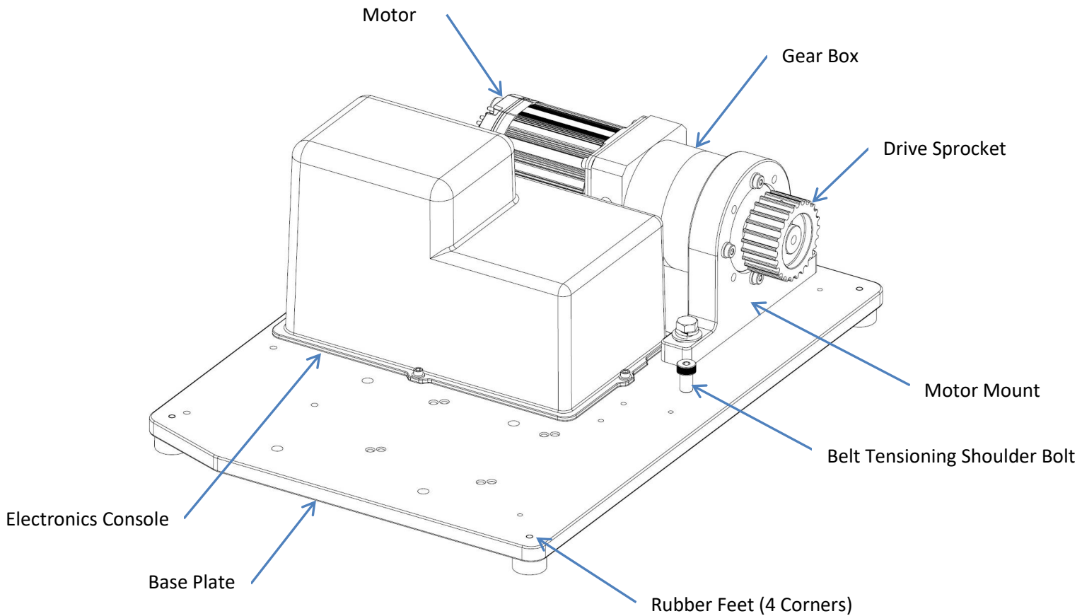
Figure 1: Major Component Overview
