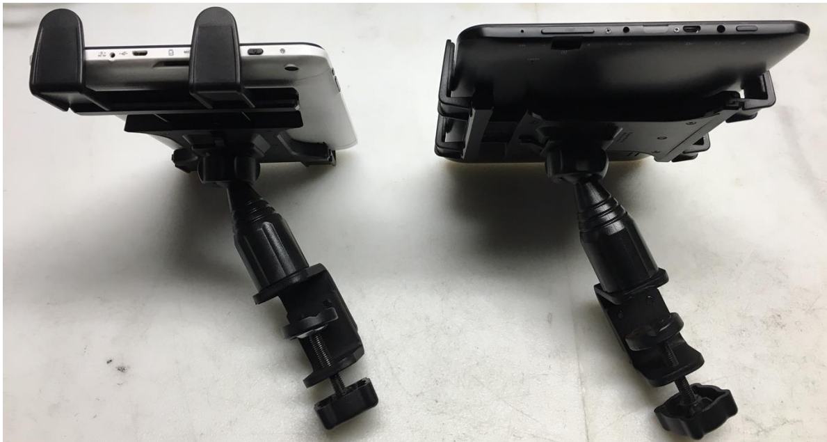
Figure 12: Side view of Tablet holder 9 inch (left) Upgraded 10 inch (Right)
