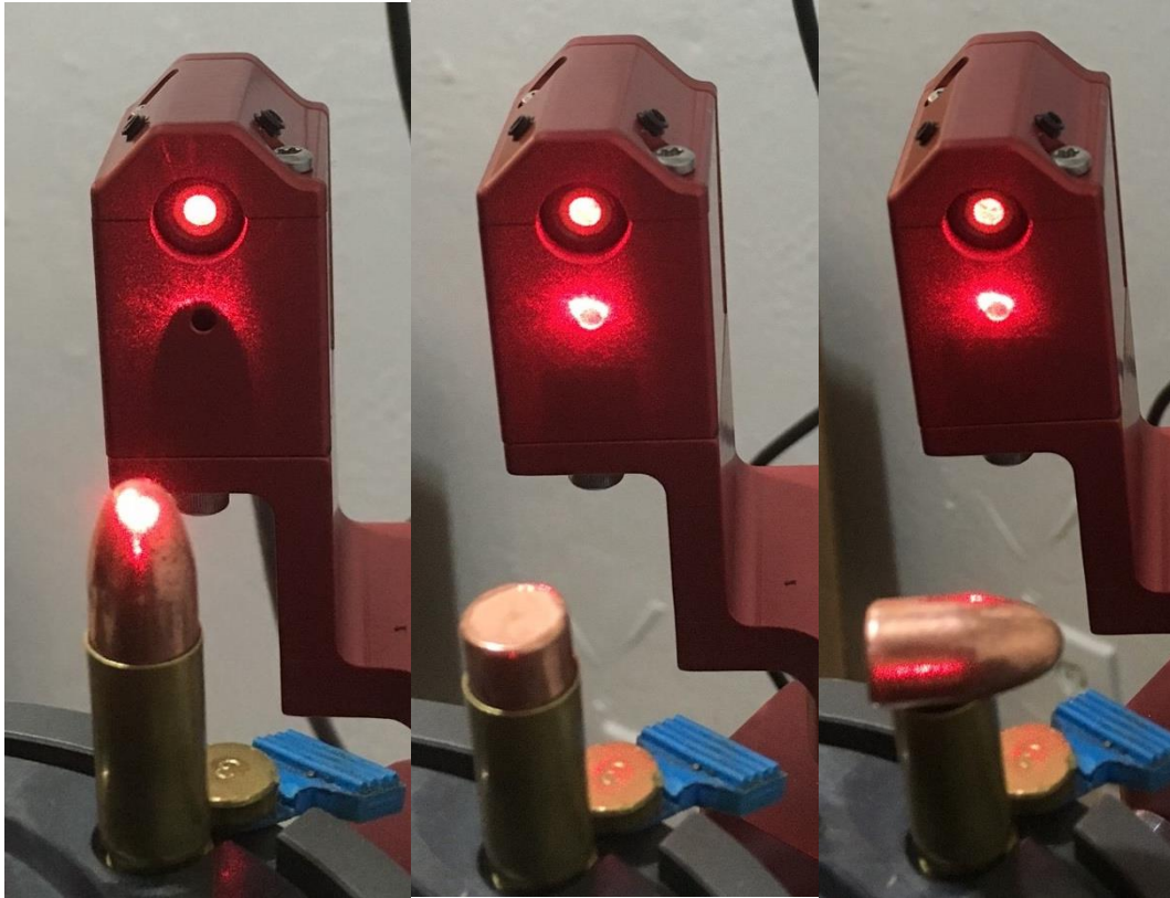
Figure 49: Properly orientated Bullet- Beam interrupted (Left) Improper orientated Bullet – Beam not interrupted (Right)
