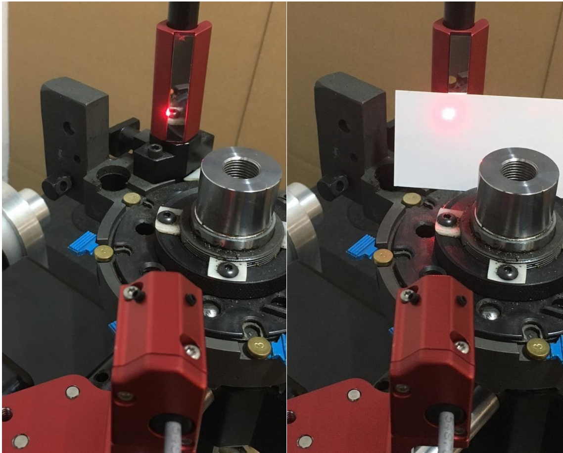
Figure 45: Laser Beam (Not aligned) directed on the edge of the mirror.
