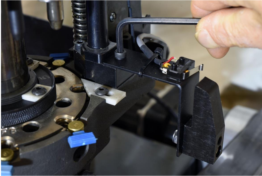
Figure 60: Installing the Shield Latch
