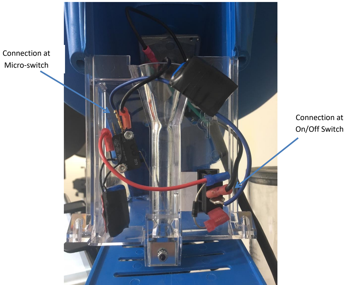
Figure 18: Case Feeder RC Filter
