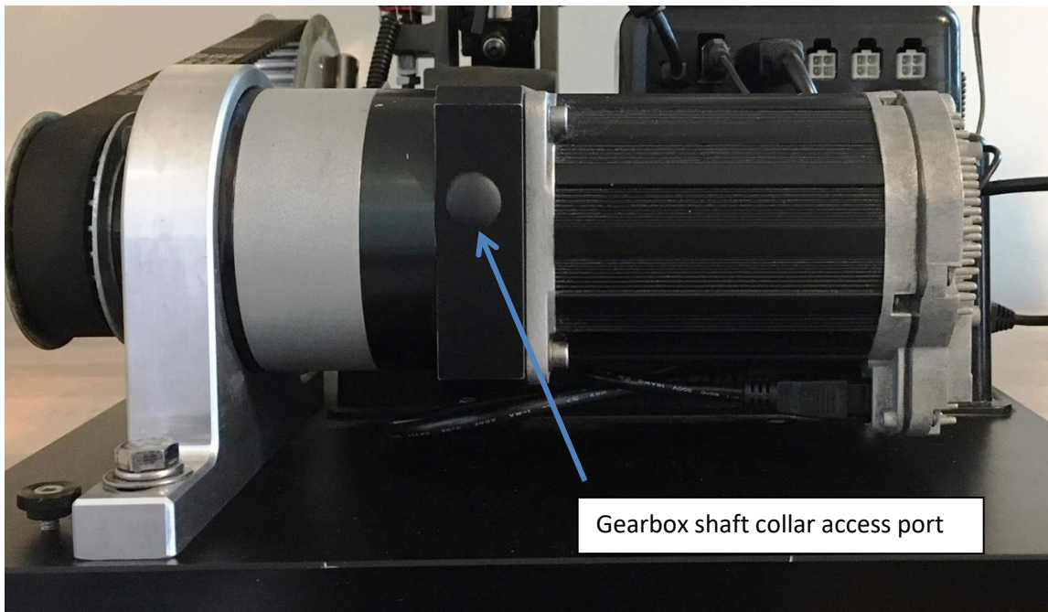
Figure 76: Gearbox Shaft connection
