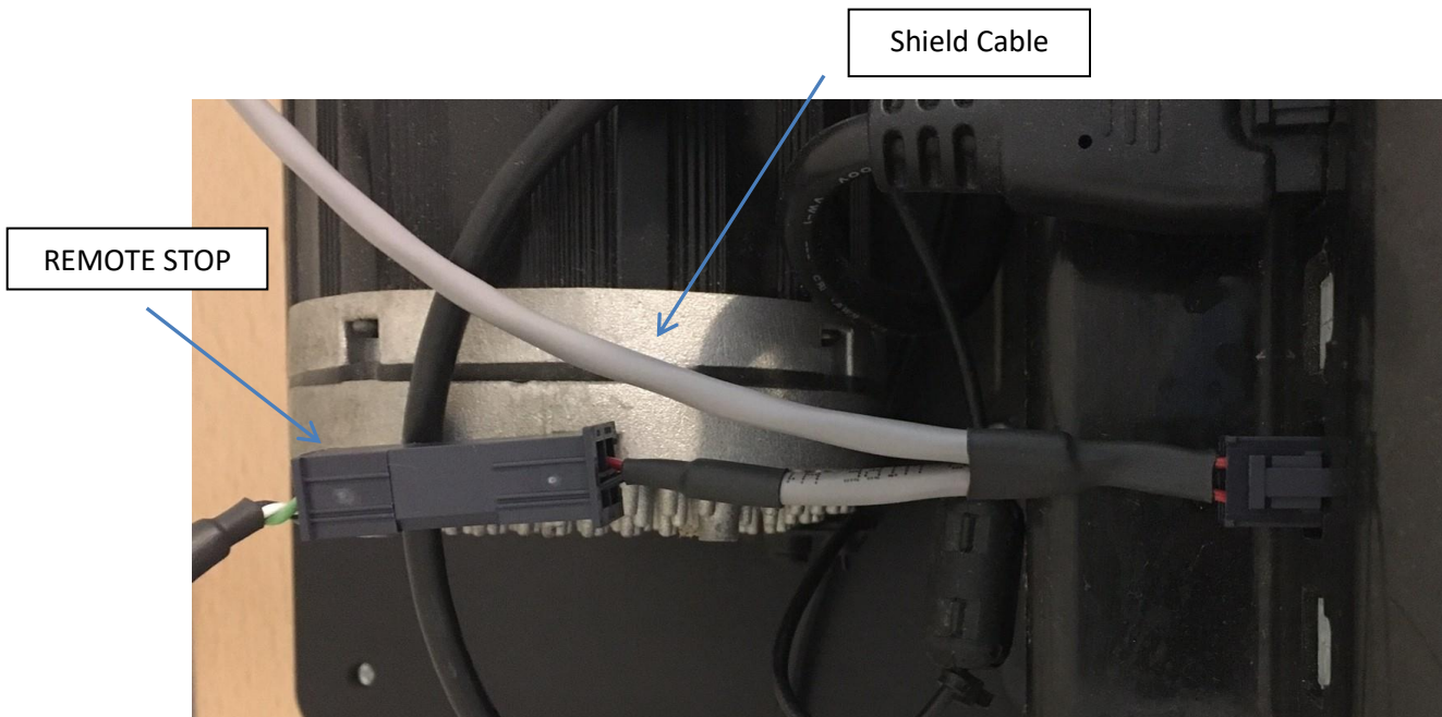
Figure 61: Cable Assembly
