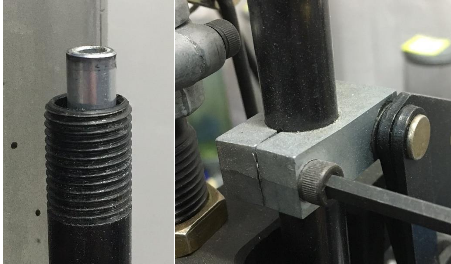
Figure 43: Removing low primer sensor and priming mechanism from priming tube
