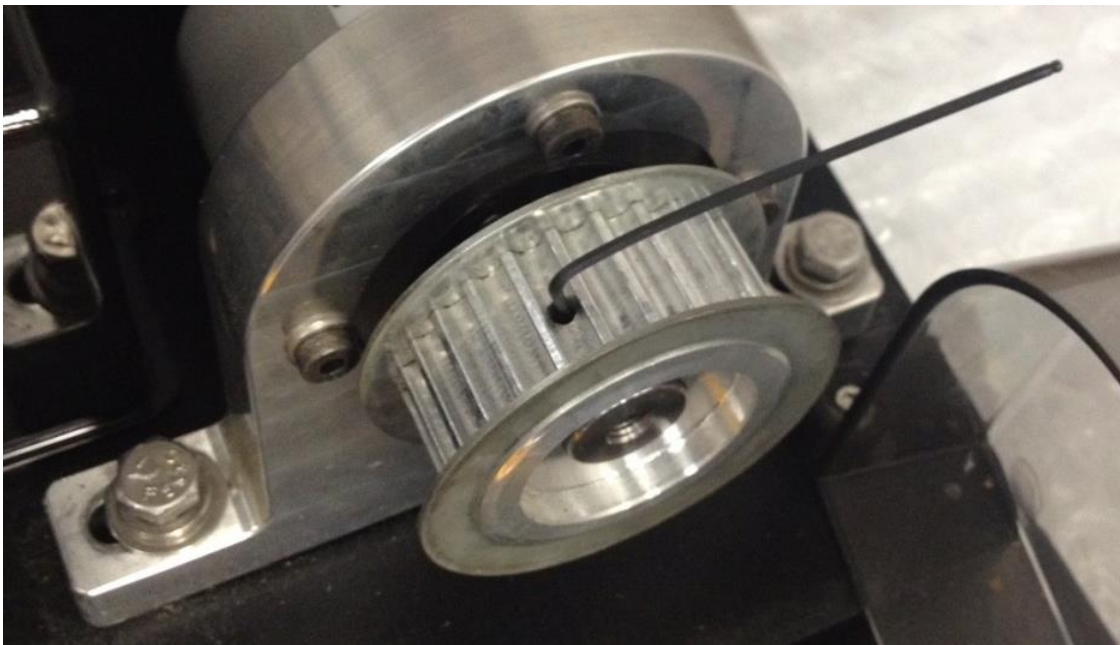
Figure 74: Adjusting the small sprocket position on the gearbox shaft
