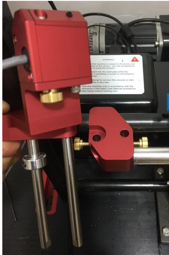
Figure 40: Removing the upper mount for station configuration change
