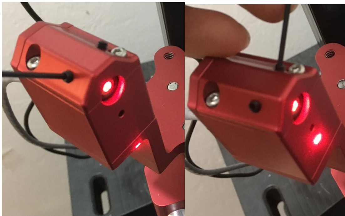
Figure 46: Adjust the set screw to align the laser. Before adjustment (Left) Mid Adjustment (Right)
