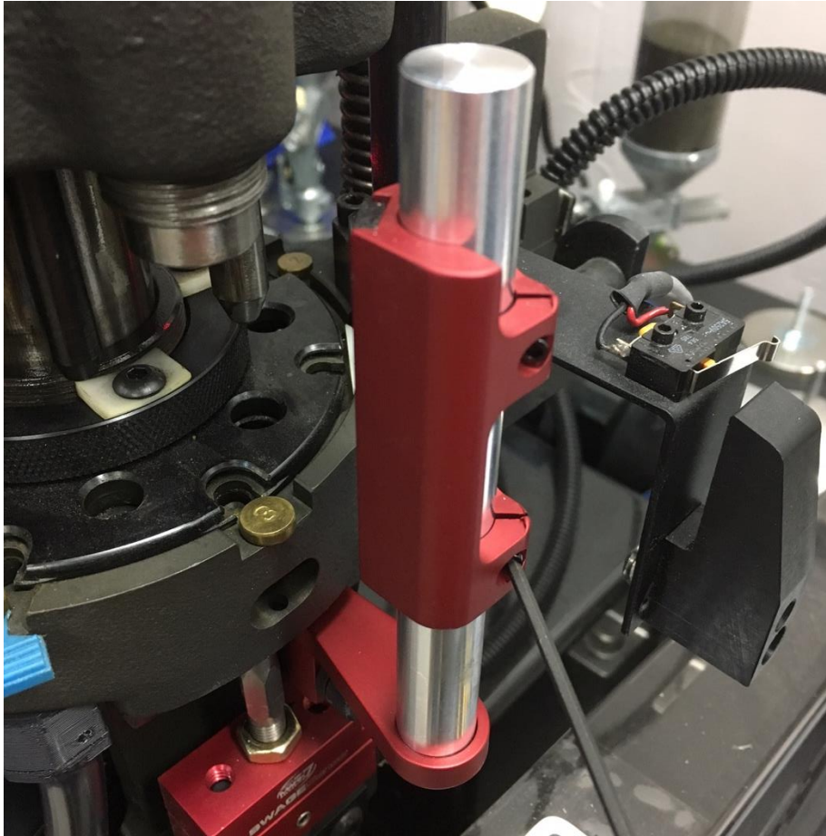
Figure 53: Mirror Mounted to Station 8 adapter rod.
