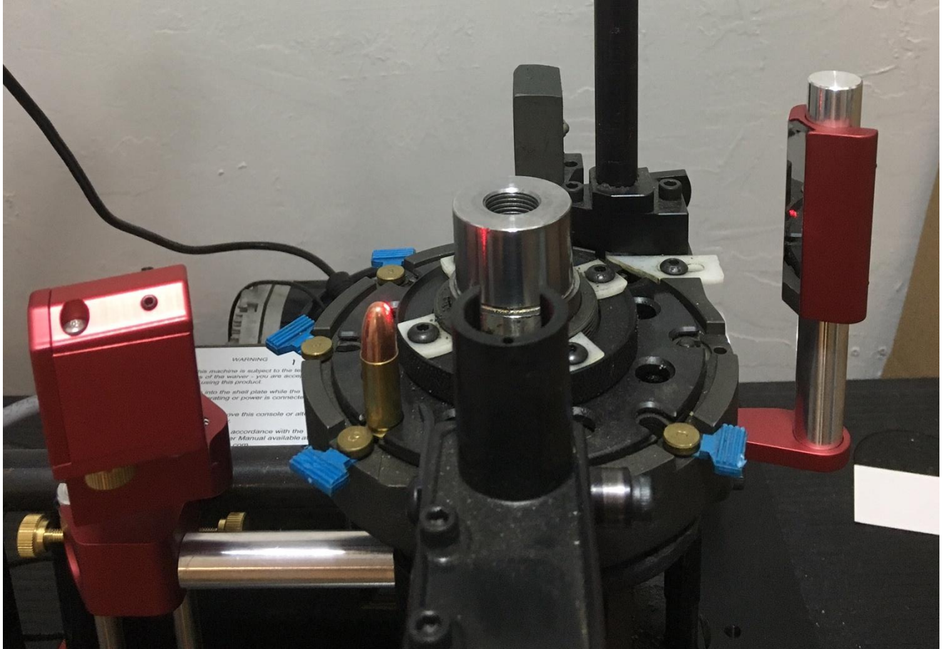
Figure 54: Station 8 Setup (tool head removed for picture)
