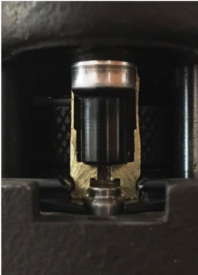
Figure 33: Cross-section of properly adjusted Swage Rod
