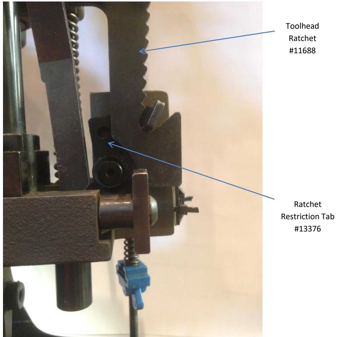
Figure 8: Removing Ratchet arm
