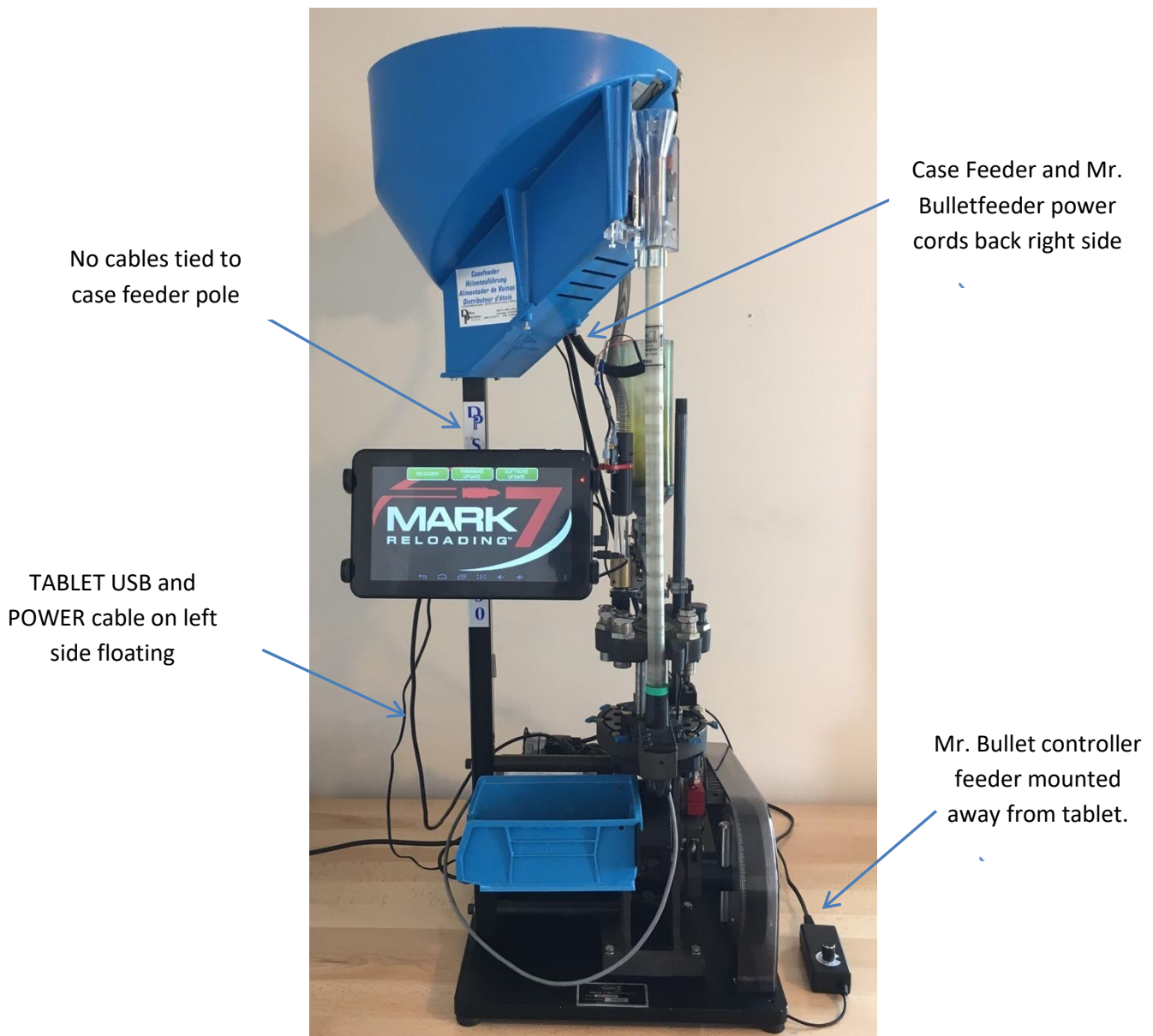
Figure 19: Recommended cable management front view
