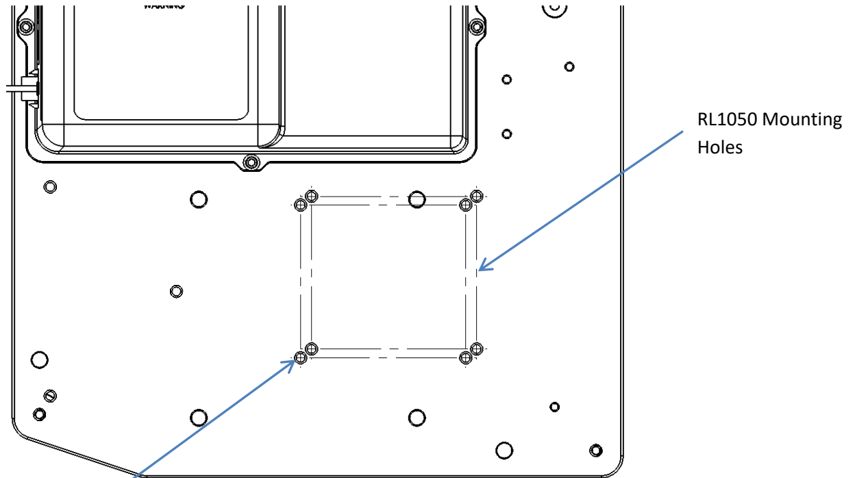
Figure 2: Mounting Location on baseplate for RL and Super
