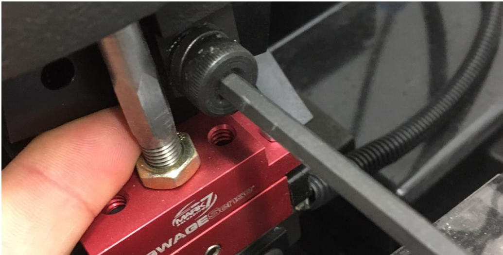
Figure 51: Removing the shoulder bolt to mount on station 8 adapter.
