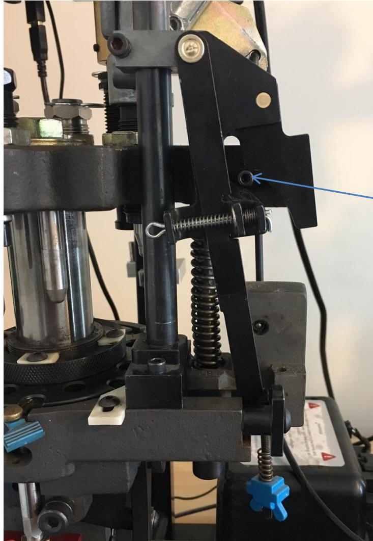
Figure 9: Ratchet mechanism removed
