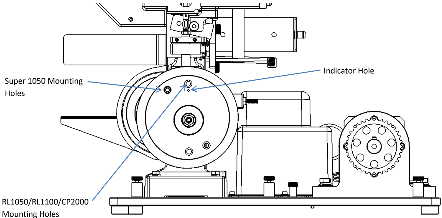
Figure 3: 1050 fastened to baseplate with large sprocket installed
