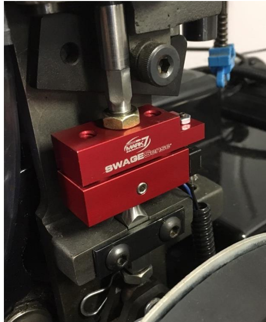
Figure 31: SwageSense® Installed
