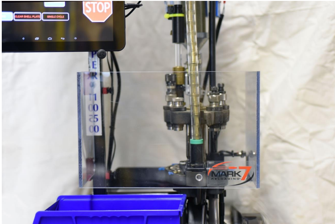
Figure 62: 1050 Shield Installed
