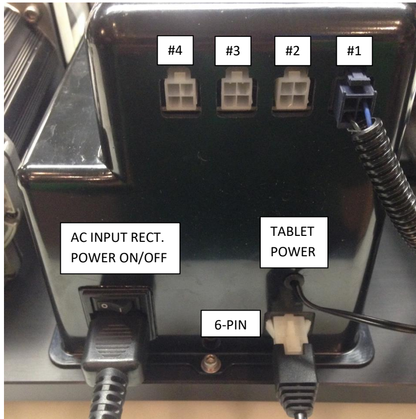
Figure 15: Side of Console Inputs
