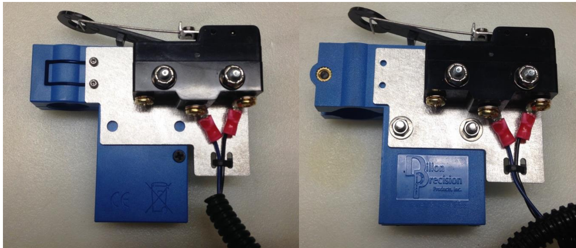
Figure 24: New Style mounted Left, Old style Mounted Right
