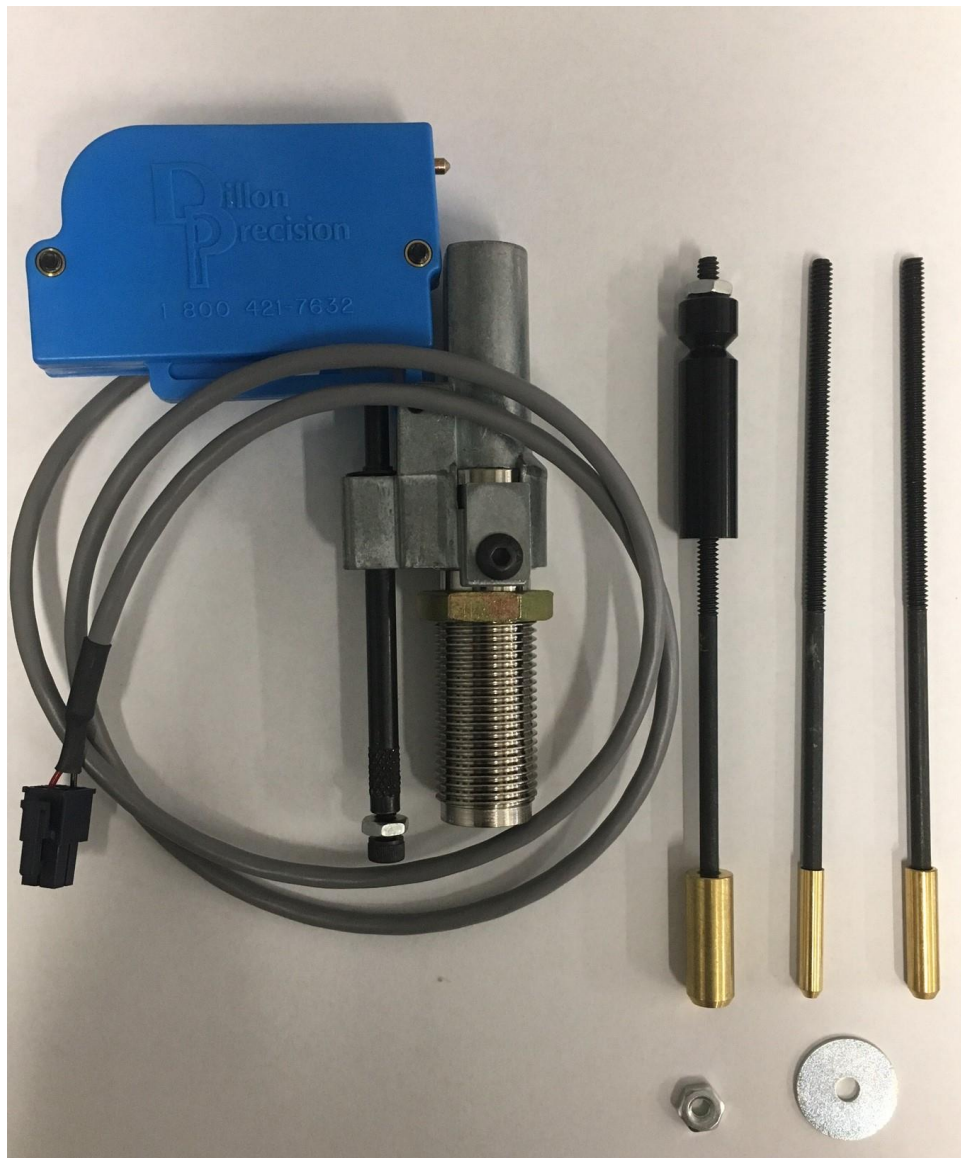
Figure 57: PowderSense® Complete Kit
