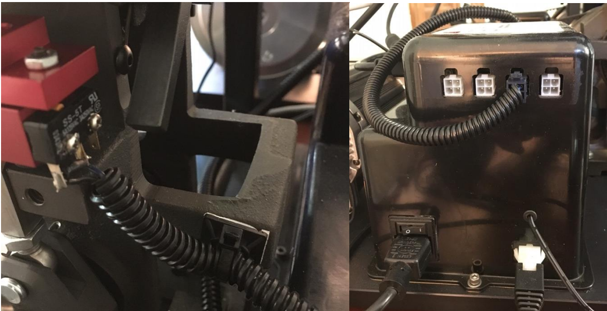
Figure 32: Cable assembly with strain relief, Port to plug into console.
