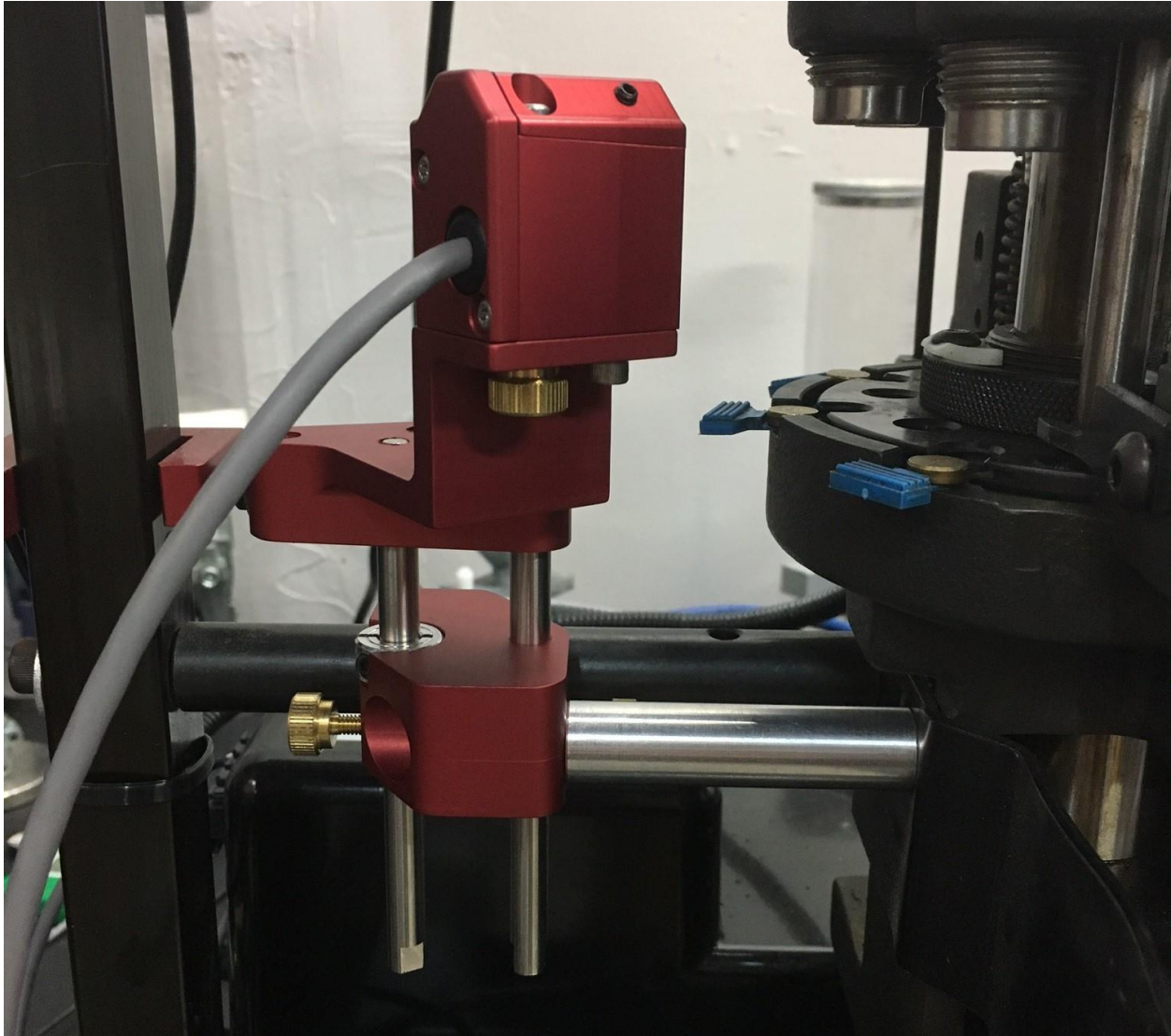
Figure 39: Mounting the Main Assembly
